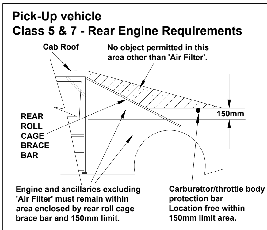
FIGURE 30 PICK-UP REQUIREMENTS.
