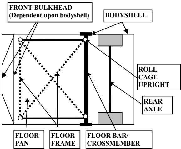
FIGURE 7 FLOOR BARS/FLOOR FRAME. Figure is diagrammatic.
