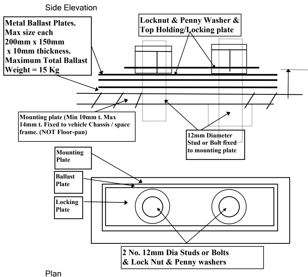
FIGURE 28 BALLAST REQUIREMENTS.
