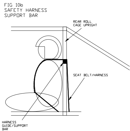
FIGURE 10 SEAT BELT HARNESS SUPPORT BAR.
