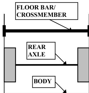
FIGURE 22 CROSS BRACE/MEMBER END PLATES.
