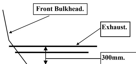
gii FIGURE 12 PERMITTED EXHAUST THROUGH BULKHEAD LOCATION.
