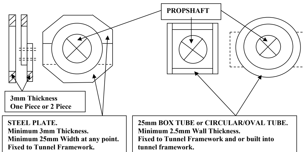
FIGURE 23 PROPSHAFT CATCH PLATE &amp; CONTAINMENT HOOPS.
