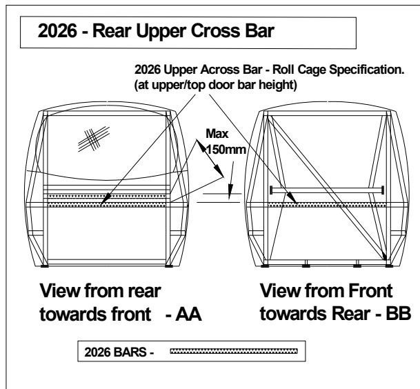
Figure 1b.iv - Roll Cage - Original Floor not Intact. 2026 – New mandatory bars. Rear Upper Cross Bar.
