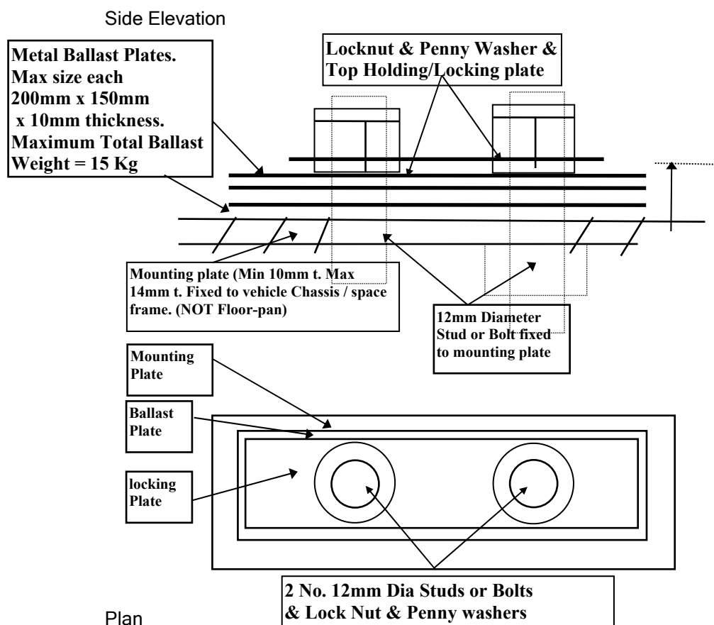
FIGURE 28 BALLAST REQUIREMENTS.
