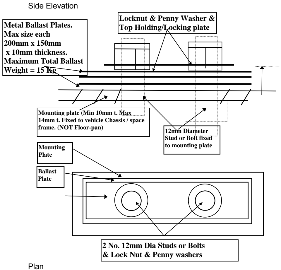
FIGURE 28 BALLAST REQUIREMENTS.
