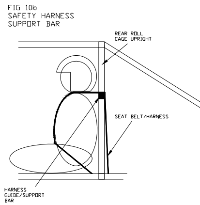
FIGURE 10 SEAT BELT HARNESS SUPPORT BAR.
